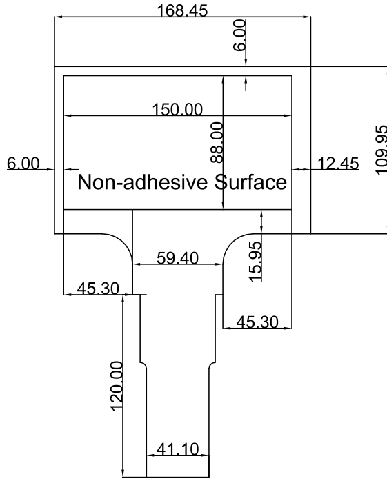
FPC FRONT
