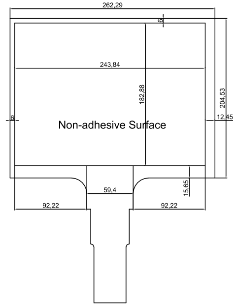
Golden Finger FRONT
