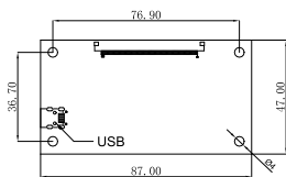
STM Controller
