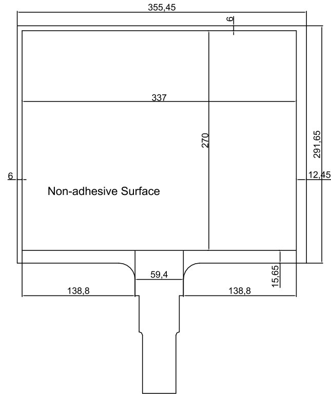
Golden Finger FRONT
