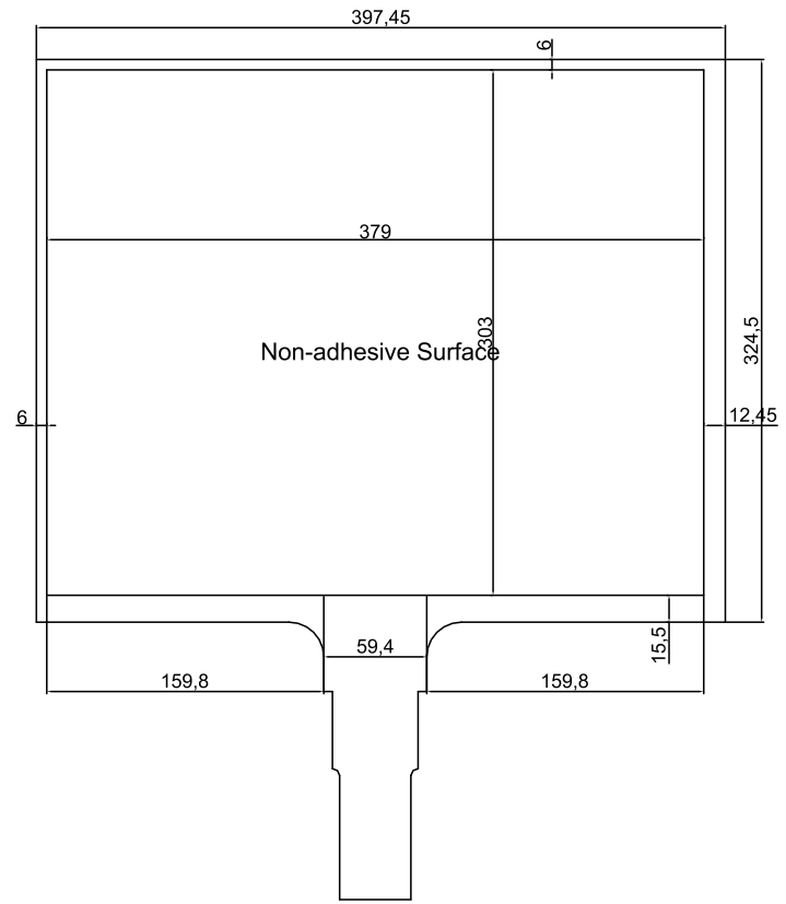
Golden Finger FRONT Effective width:379.00;Effective height:303.00;Cutting width:397.45;Cutting height:324.50
