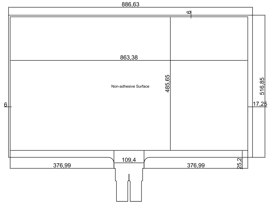
Golden Finger FRONT Effective width:863.38;Effective height:485.65;Cutting width:886.63;Cutting height:516.85
