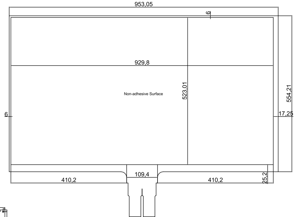
Golden Finger FRONT
